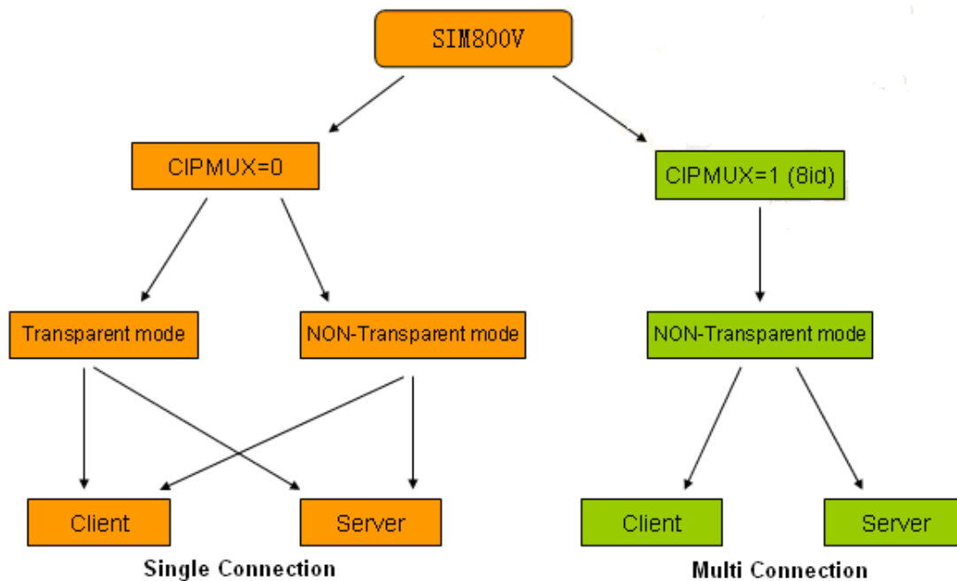
Figure1: SIM800 series TCPIP Structure
