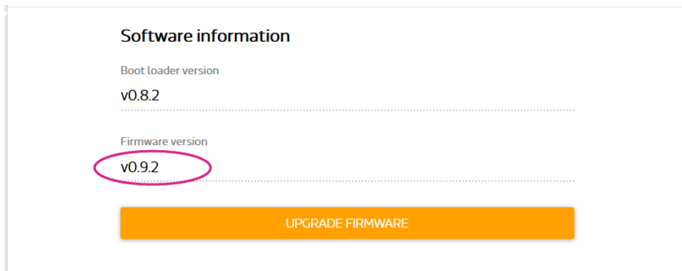
Figure 8 Firmware version
